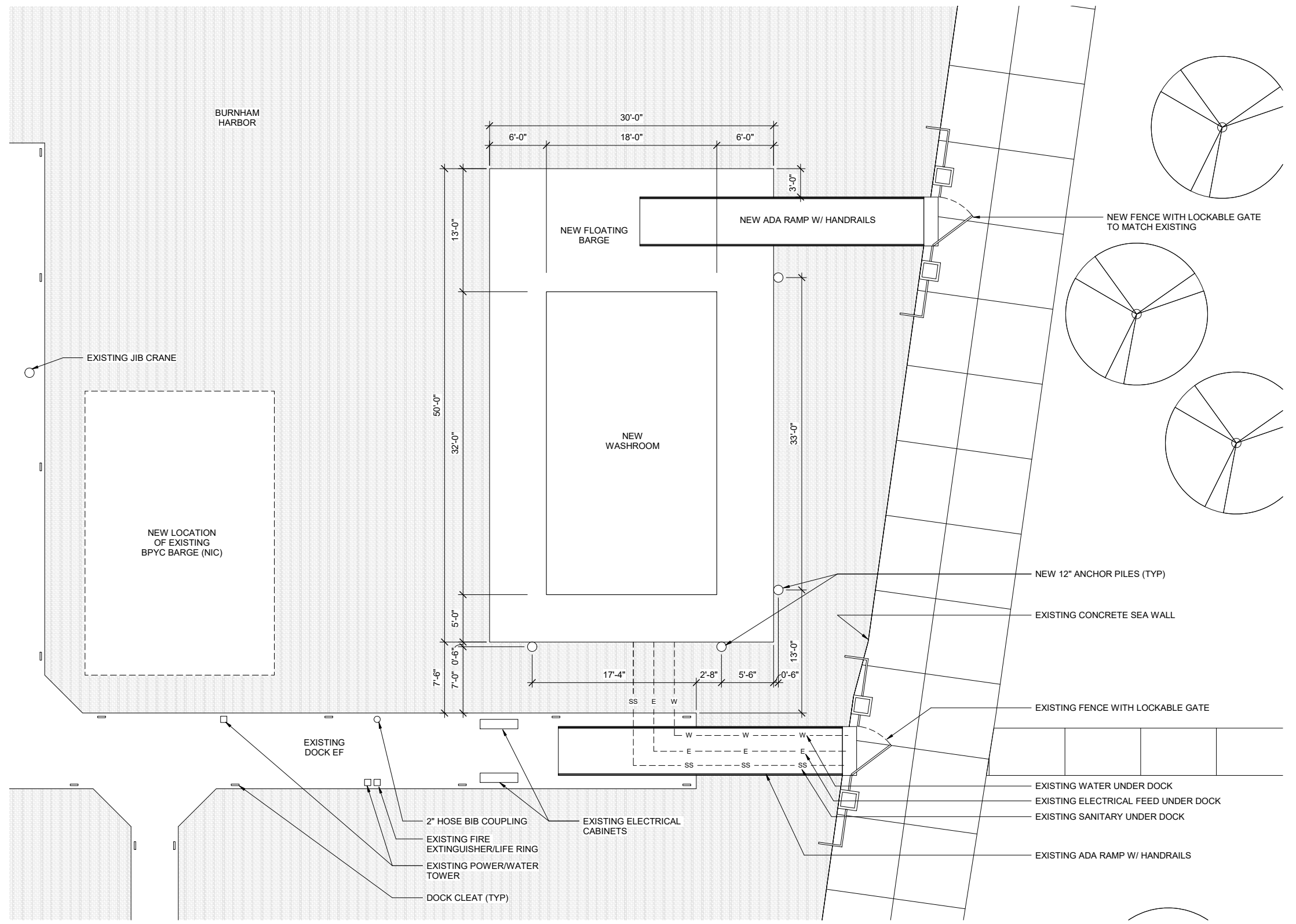
1 PLATFORM LOCATION PLAN - BURNHAM HARBOR DOCK EF N.T.S.
